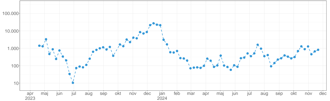
Wastewater concentration of SARS-CoV-2, Holbæk (R)
